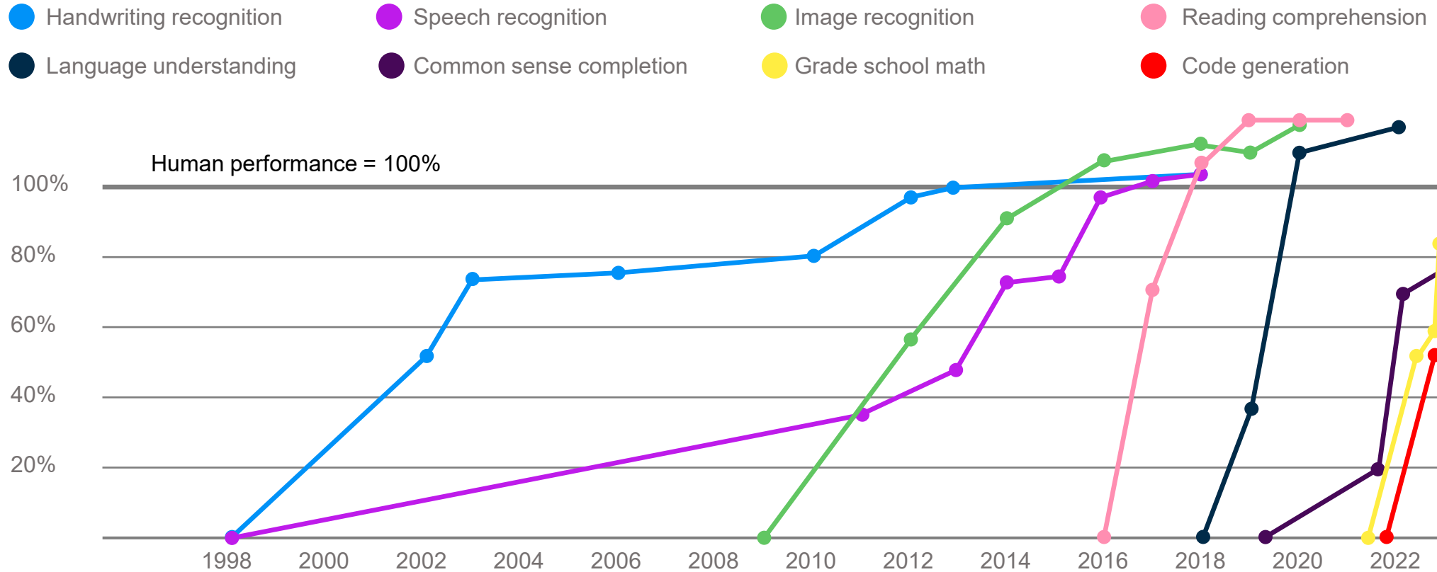
State-of-the-art AI performance on benchmarks, relative to human performance
